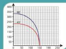
Cutting Chart - 500
