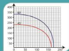
Cutting Chart - 550
