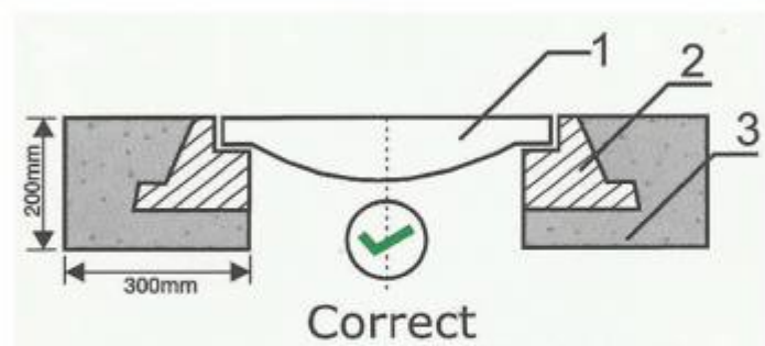
1. Manhole Cover 2. Frame 3 M-20 Grade Concrete
