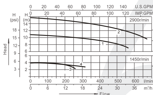
Performance curves:
