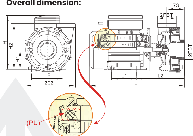
Overall dimension:
