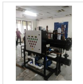
Water Cooled Scroll Chiller
