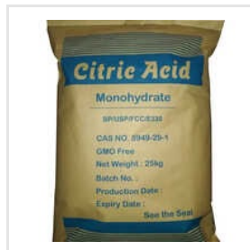
Monohydrate Citric Acid
