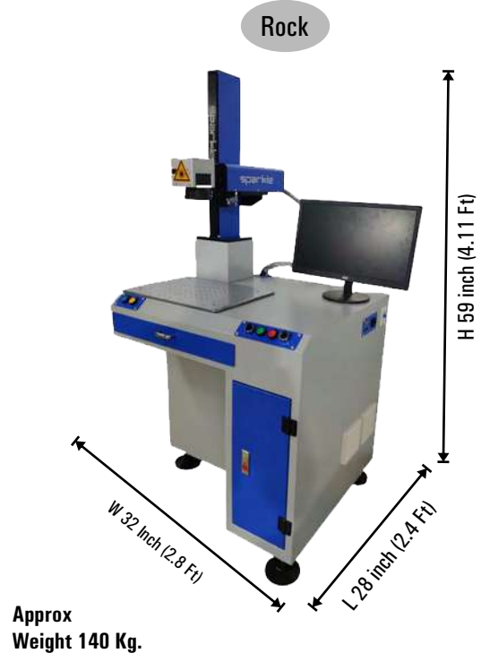
REGULAR WORK TABLE WITH HEAD UP-DOWN
