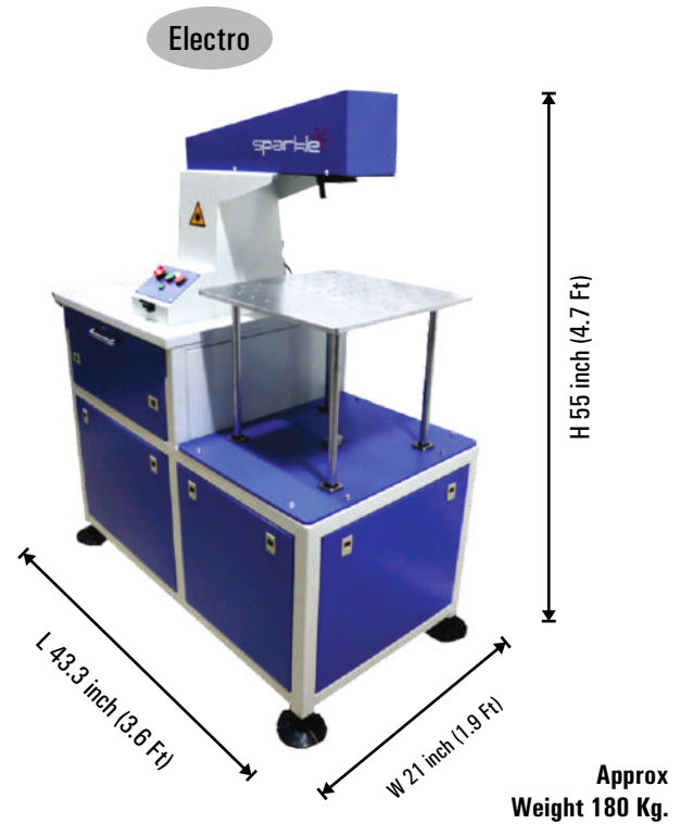
REGULAR WORK TABLE UP-DOWN & FIXED HEAD
