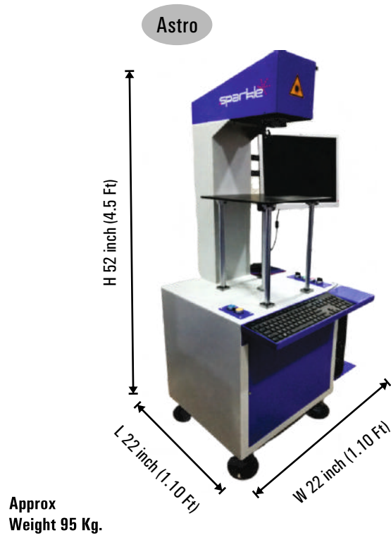
COMPACT WORK TABLE UP-DOWN & FIXED HEAD
