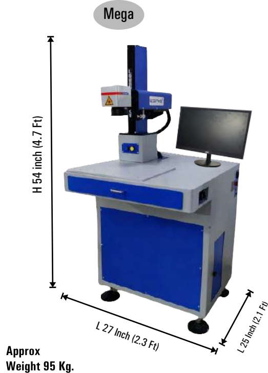
COMPACT HEAD UP-DOWN & FIXED HEAD WORK TABLE
