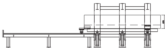
CORNER HYDRAULIC PRESS 1 Daylight 1 Trolley
