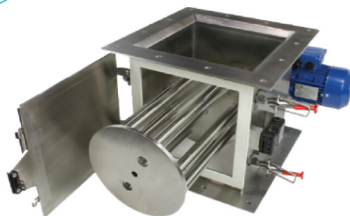
Rotary Magnet
