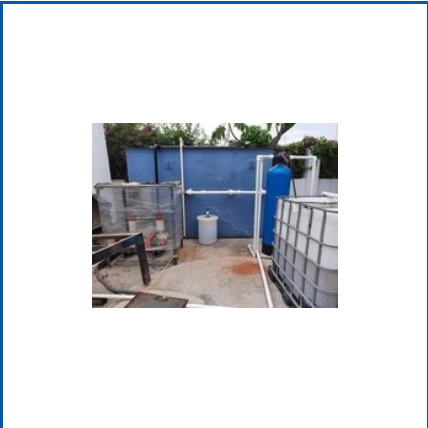
MBBR BASED PACKAGED SEWAGE TREATMENT PLANT
