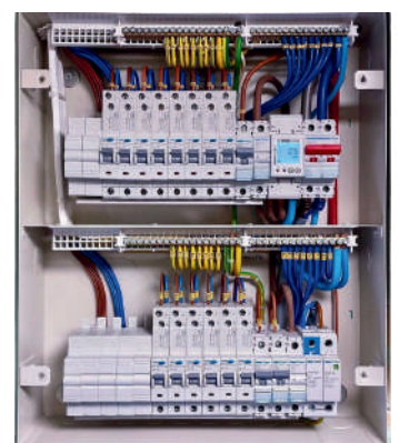
ELECTRICAL PANEL
