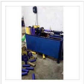
Paper Tube Bend Nosing Machine
