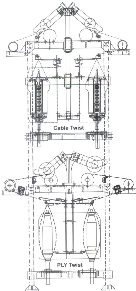
Yarn Path
