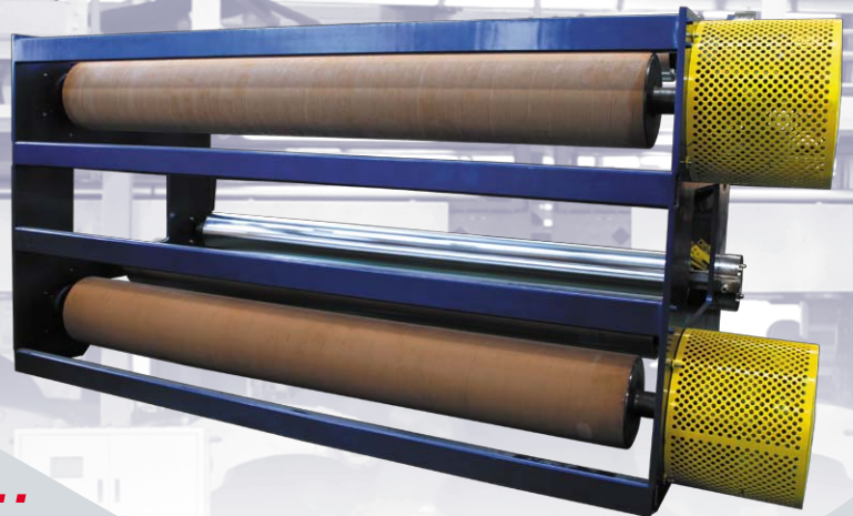
High speed servo steering device
