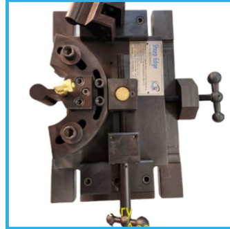
ROTARY MOUNTING UNIT DESIGN 1
