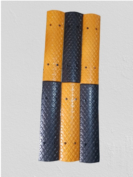
Rubber Rumbler Size- 500*125*25 mm
