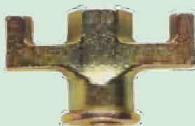
Wing Nut Malleable Cast Iron Suitable for 16 mm Dia Tie Rod
