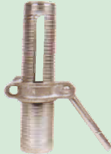
Heavy Duty Prop Sleeve Roll threaded Available in (3.0)mm thickness 200-300 mm length
