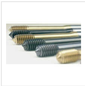
Roll Forming Taps
