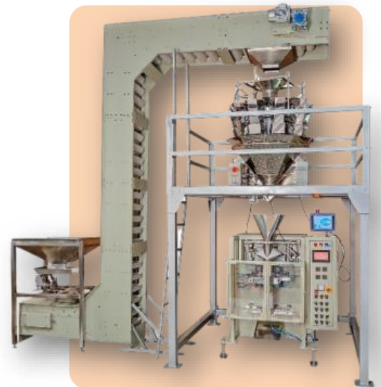
MULTIHEAD WEIGHER POUCH PACKAGING MACHINE
