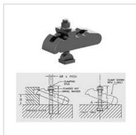
Mould Clamps
