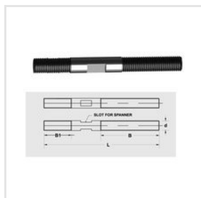
Stud With Slot (Mould Stud)
