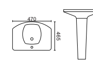
KAIZER Pedestal Basin 470 x 465 x 691 MM
