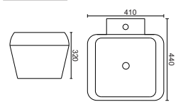
BERRY Wall Hung Basin 440x 410 x 320 MM
