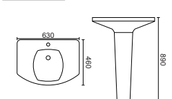
COLADO Pedestal Basin 630 x 460 x 890 MM
