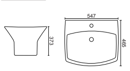
RAPPORT Wall Hung Basin 547 x 465 x 373 MM
