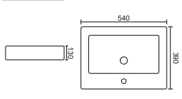
ELLIPS Wall Hung Basin 540 x 390 x 130 MM
