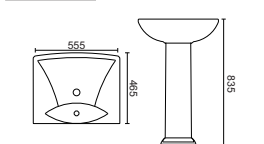
SQUARE Pedestal Basin 555 x 465 x 835 MM
