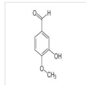
Iovanillin Compound
