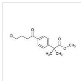
Methyl 2-(4-Chlorobutanoyl)-4-Chlorobutanoate
