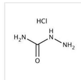
Semicarbazide Hydrochloride
