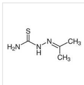
Acetone Thiosemicarbazone
