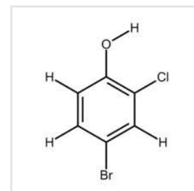
4-Bromo 3-Chlorophenol
