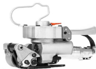
Pneumatic Pet Strapping Tool
