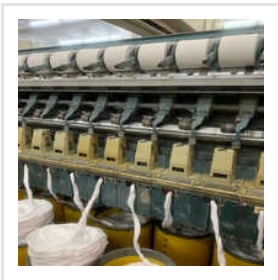
Elitex BD 200RN Carding Machin
