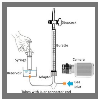
Gas Measuring Burette
