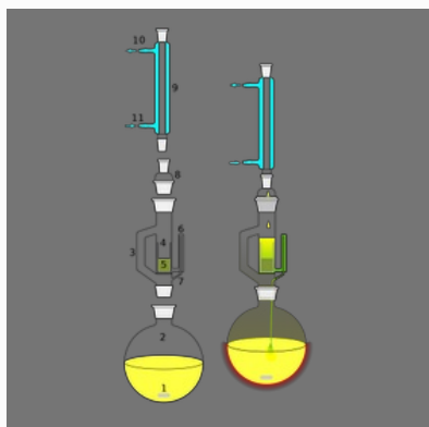
soxhlet extraction apparatus
