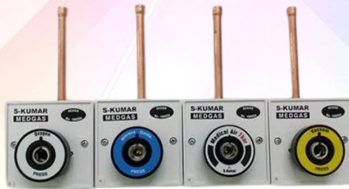
Suction Regulator & Medical Gas Outlet
