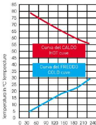
TEMPERATURE CURVE
