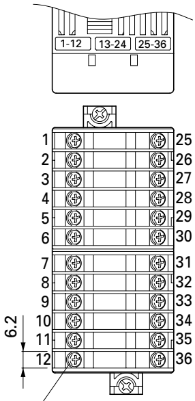
Terminal screw M3
